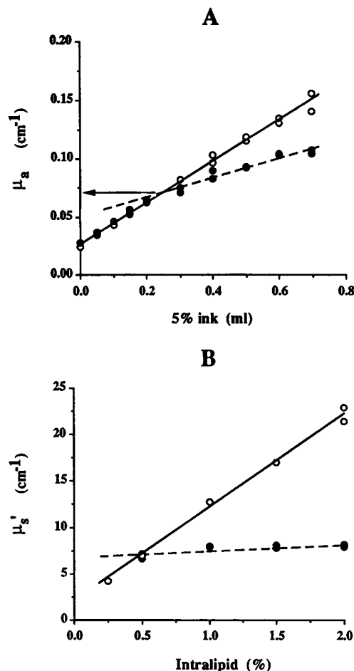
FIGURE 1 Determination of the absorption and the reduced scattering coefficients of isolated mitochondria. TRS was performed without (○) and with (●) the sample bag (12 mg protein/ml) as described in Materials and Methods. Each experimental point represents one TRS spectrum acquisition. (A) Example of the \mu_a determination of isolated mitochondria by the substitution method. Arrow indicates the value of the \mu_a corresponding to the "break point" of the dashed line. (B) Example of determination of the \mu_s' of isolated mitochondria by the substitution method.
