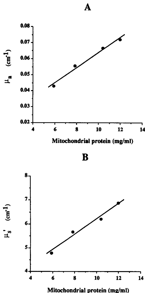
FIGURE 2 Relationship between the absorption and reduced scattering coefficients and the concentration of isolated mitochondria. The absorption ( A ) and the scattering ( B ) coefficients were determined by using TRS and the substitution method as described in Fig. 1, A and B , and in Materials and Methods.
